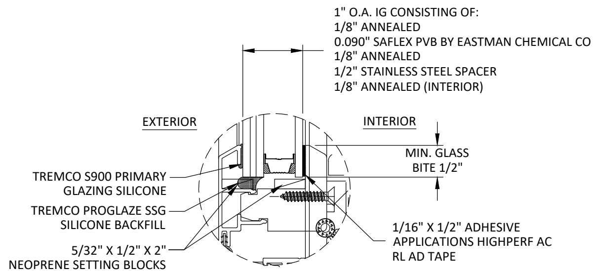
G1 GLAZING DETAIL
