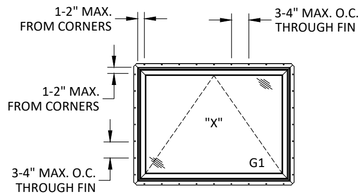
ANCHOR LAYOUT NAIL FIN INSTALLATION
