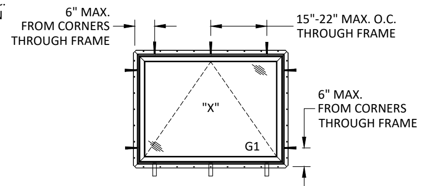
ANCHOR LAYOUT THROUGH FRAME + STRAP INSTALLATION
