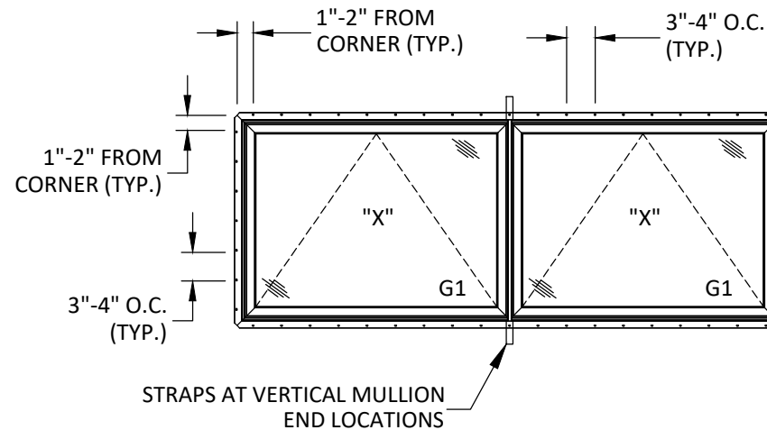
ANCHOR LAYOUT NAIL FIN AND STRAP
